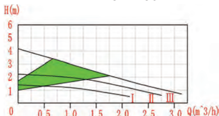
AM-EAC25-4-130
