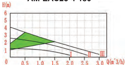
AM-EAC25-4-180
