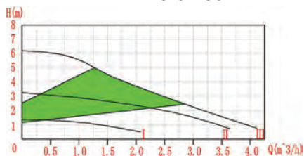
AM-EAC25-6-130
